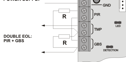
Example of wiring the JS-25 into the double EOL zone.
